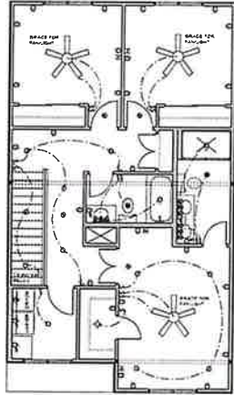
SECOND LEVEL ELECTRICAL PLAN SCALE: 1/8" = 1'-0"
