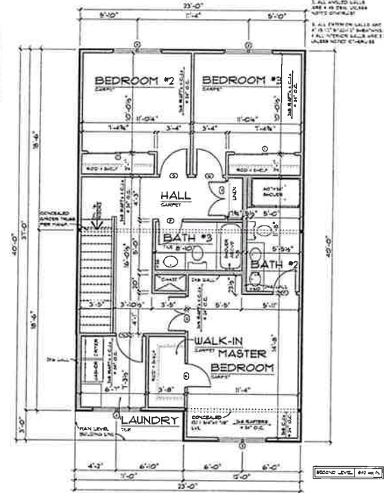
SECOND LEVEL FLOOR PLAN SCALE: 1/8" = 1'-0"
